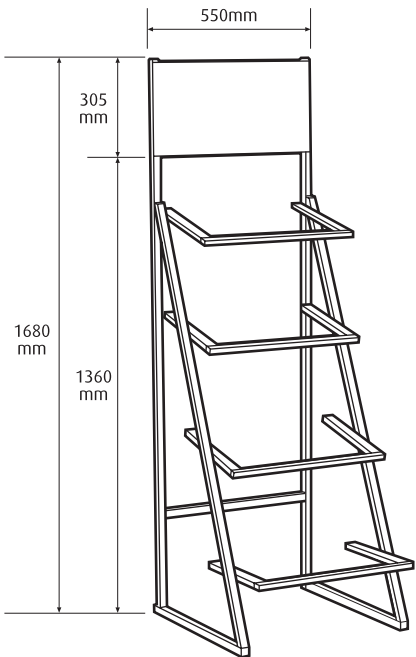
No. 968 Freestanding Frame for Special Offer Bins
